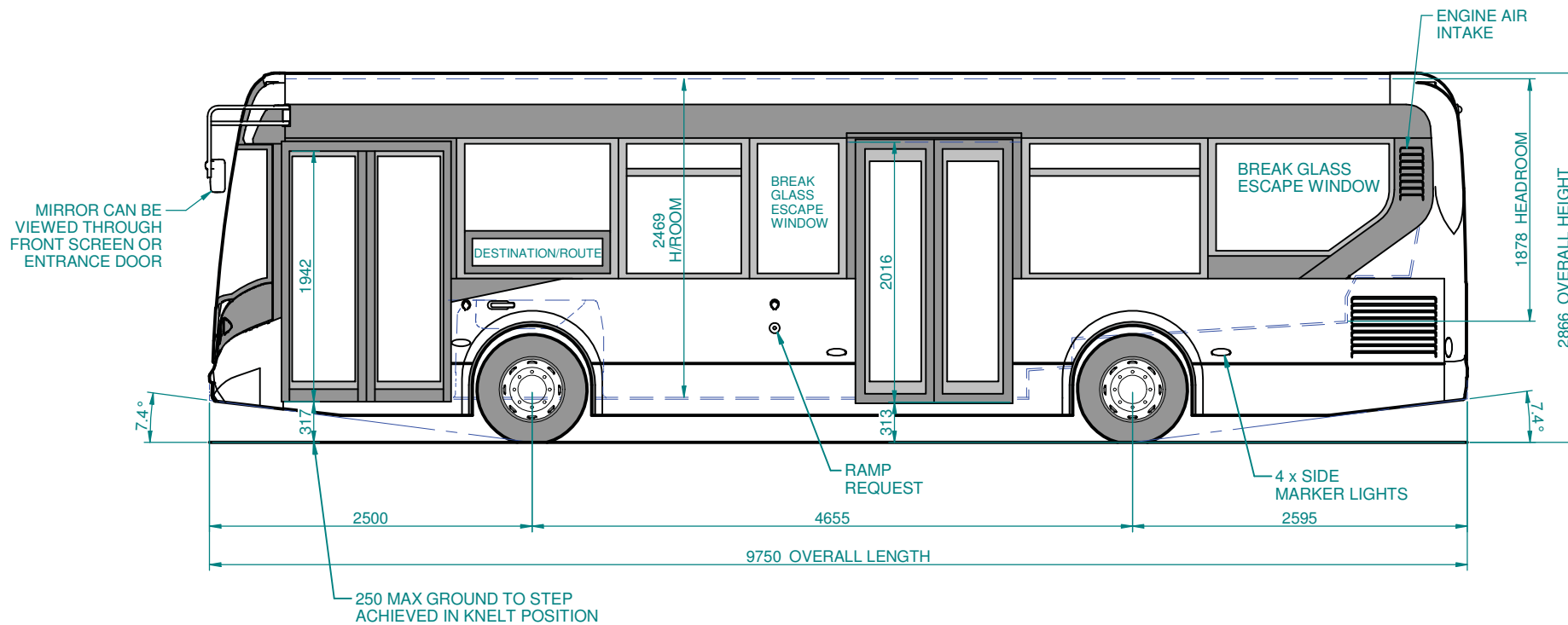
LEFTHAND ELEVATION
